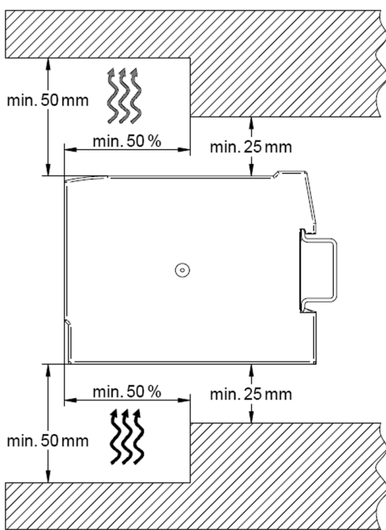
Bild 2: Einbau Figure 2: Installation Figure 2: Montage Figura 2: Incasso Figura 2: Montaje
