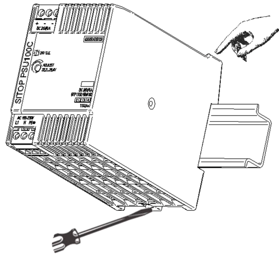
Bild 3: Montage Figure 3: Mounting Figure 3: Fixation Figura 3: Montaggio Figura 3: Montaje
